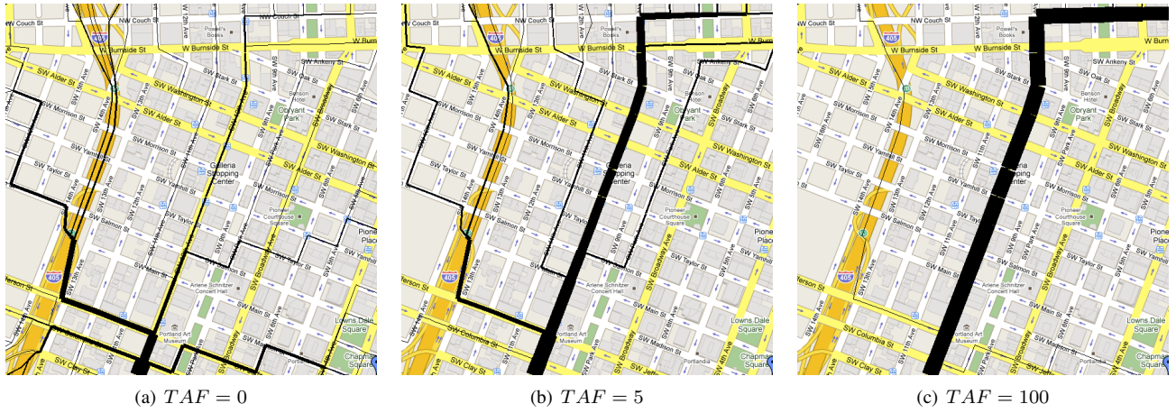
Fig. 2. Example of path generation from a single source for different values of the Trip Aggregation Factor TAF . The thickness of the segment represents the number of paths traversing it.
